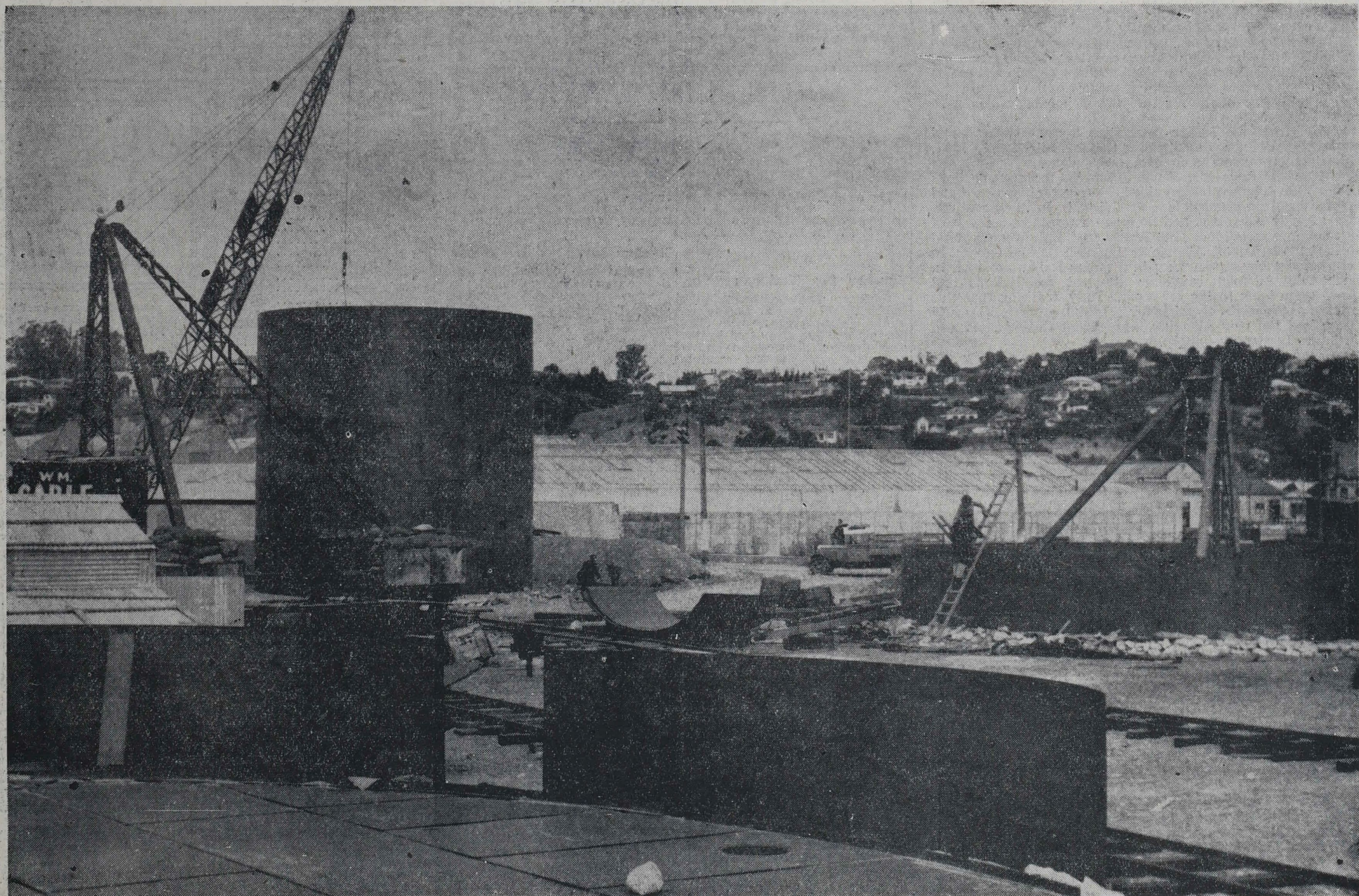
NEW STORAGE TANKS AT PORT AHURIRI.—A general view of the work in progress at the Port. The Vacuum Oil Company, Ltd., is erecting four huge storage tanks with a total capacity of 2,750,000 gallons, utilising the latest methods of construction. The tanks, which will be ready for use about September, will cost about £17,800, and the new administration buildings about £13,000.
