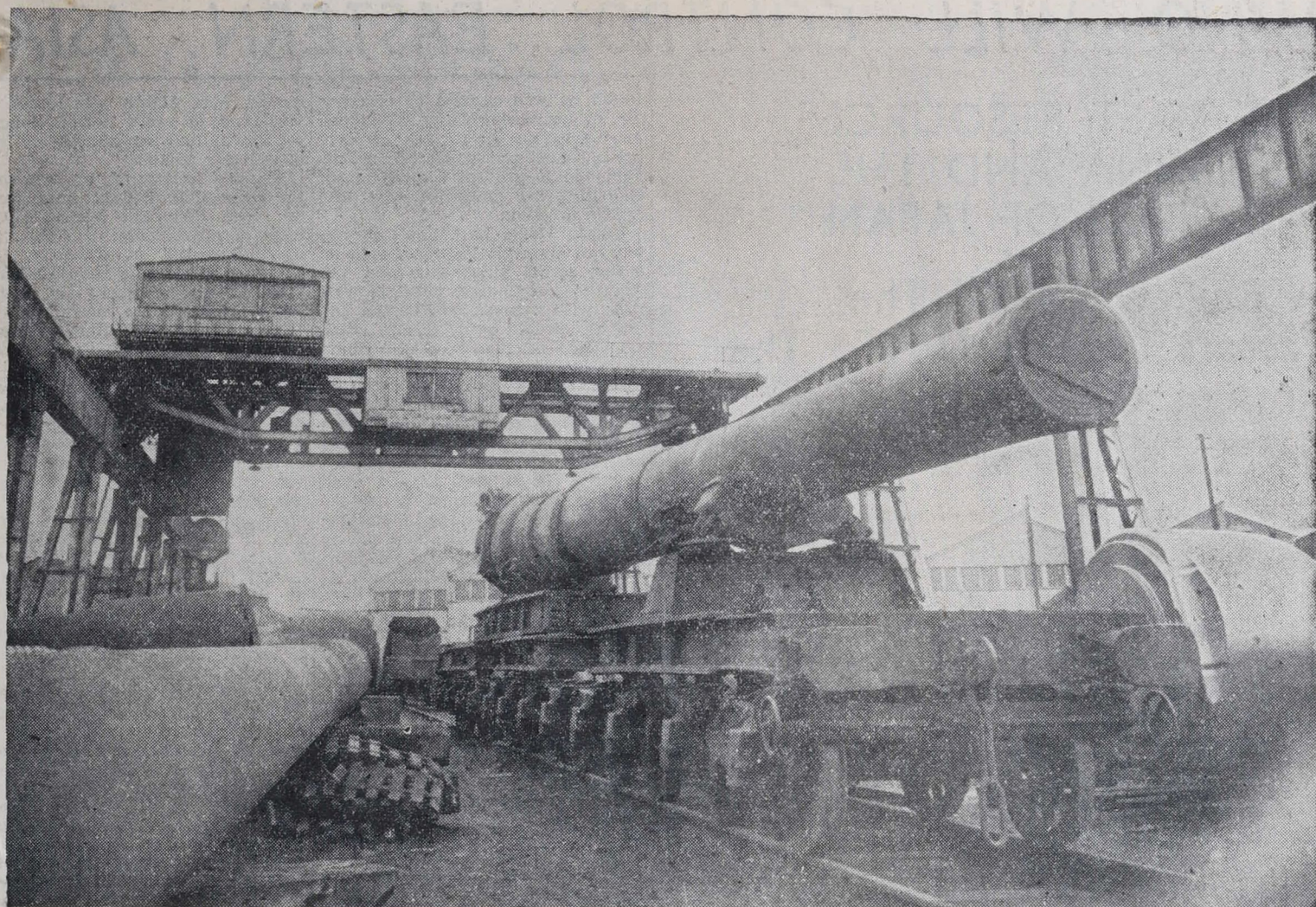
REPAIRING 15 AND 16 INCH NAVAL GUNS AT WOOLWICH ARSENAL.—Sixteen-inch guns on a railway truck ready for removal by rail.
