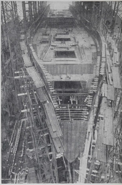
THE N.Z. BIRMINGHAM WORKS IN COURSE OF CONSTRUCTION FOR THE SHAW BAYLI & SIBSON CO., LTD., AT THE YARD OF HARRIS WAY BENTON & WINDUS ENGINEERING LTD., WALLING-ON-THE-TAHEA, OF COURSE A 100 FT. FROM THE BOW TO THE STERN.
