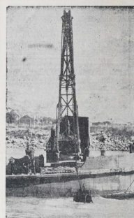
DREDGING UNDER WAY.—The Napier Harbour Board's dredge at work.
