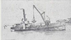
NAPIER HARBOUR WORK.—The Napier Harbour Board's dredge at work on the inner harbour following the recommendation made by the director of Harbours.
