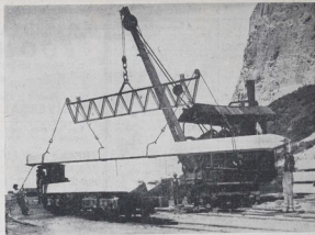
A NEW WHARF PILE —A crane is shown loading a pile on its tracks at the Breakwater, Napier. The pile are destined for the new wharf.
