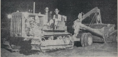
NIGHT WORK AT PAKOHIA.—A modern powerful inter-portal tractor makes light work of building a stopbank. The work is proceeding without a stop and should be completed soon.
