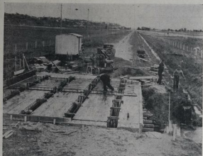
BRIDGE BUILDERS AT WORK. —Recently Road extension, the new main route from Napier through Napier to Carterton and Pukekohe, will be opened when the Intermediate bridge shown in the picture is completed. The route will, among other things, relieve the congestion of traffic from Napier to the coast.
