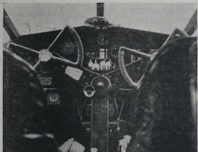
AS SEEN BY THE PILOT. —The completed instrument panel of the Union Aircraft D.H. 60 express six-seater Komatiks, which operates between Gisborne and Christchurch. The machine, which has four engines, carries many maps and necessary wireless equipment, is daily serviced.
