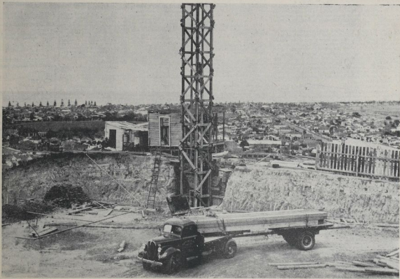
THE NEW NAPIER RESERVOIR —The excavator sunk is now complete and everything is in readiness for laying the concrete, for which purpose the large towers seen in the picture will be used. Mason Park is seen on the left, and Paper Bush on the right.
