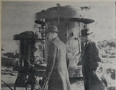
SAVAGER GEAR FOR THE PORT BOWEN. —Mr. J. Brown, of the Railway Marine Underwriters and Salvage Association (left) and Captain D. H. Gilson, of the Port Louis Salvage Office, inspect salvager gear, including the two portable beam cranes, at Charlton's yard.
