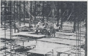
RAPID PROGRESS OF PAPER RESERVOIR —Workers are seen operating the floor of the new paper reservoir. The reservoir area follows will support the solid concrete covering.
