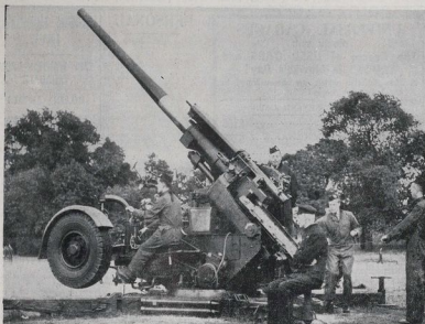
BRITAIN'S AIR DEFENCES —Large-scale air manoeuvres have been carried out during the last few days in this Britain's attacking force and air defences. Here is seen one of the most modern types of anti-aircraft gun, which protects London in the defence of London.
